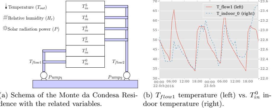
Fig. 2: Monte da Condesa schema and sample representation of indoor and water temperatures.
